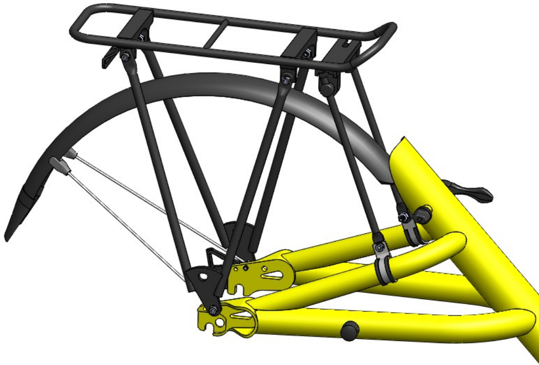
Assembly at drop outs, same both sides
