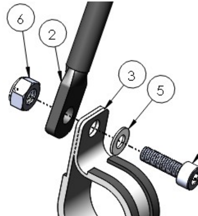
Tube Clamp Assembly
