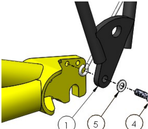
Assembly at drop outs, same both sides
